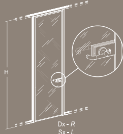
Porta anta battente vetro Single hinged glass door
