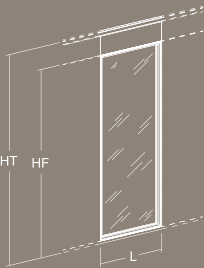
Moduli divisori vetro Glass partitions
