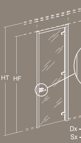
Porta anta battente vetro Single hinged glass door
