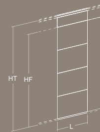
Moduli divisori ciechi a mattonella Panelled "bricks shaped" partitions
